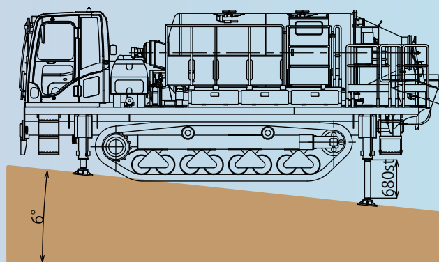
TGM-CIG500T
